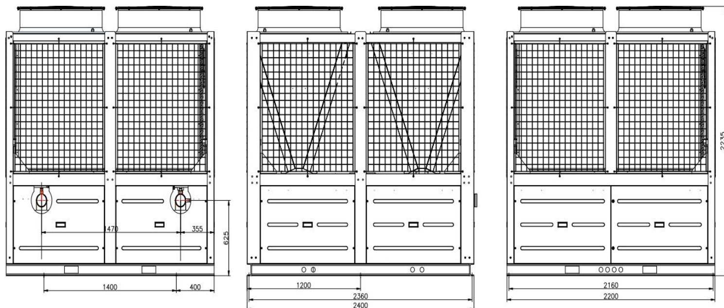
SCAW-M 260 ZHT
