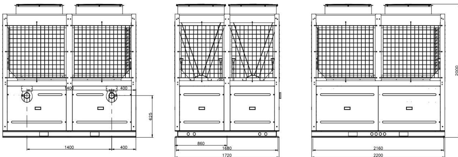
SCAW-M 165 ZHT
